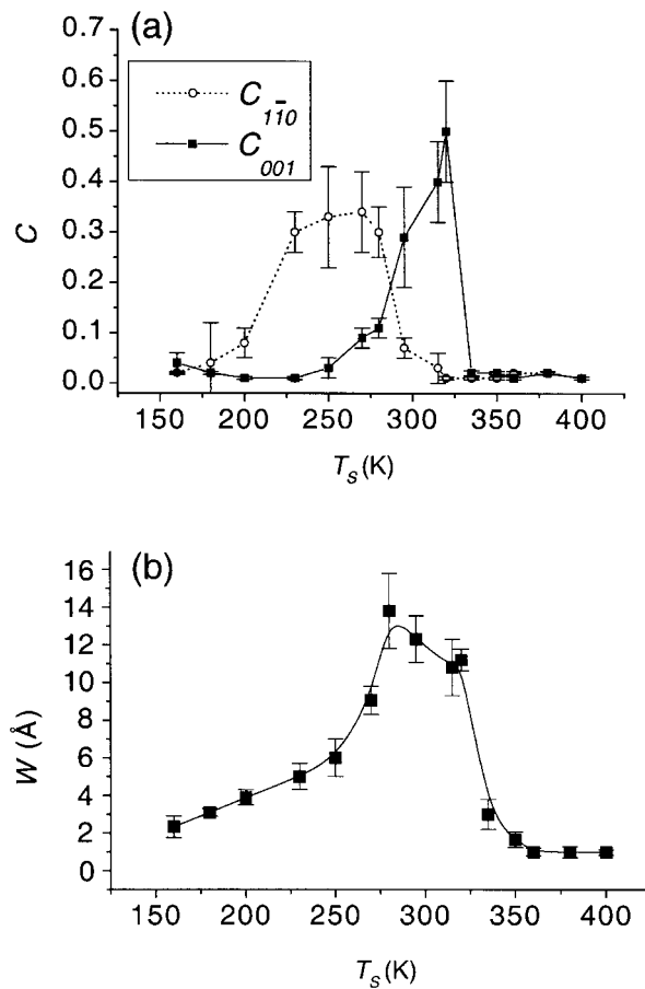
Figure 5. Surface coherence C along \langle 001 \rangle ( C_{001} ) and along \langle 1\bar{1}0 \rangle ( C_{1\bar{1}0} ) (a) and surface roughness W (b) as a function of the substrate temperature on Ag(110) after sputtering at \Phi = 4 \mu\text{A cm}^{-2} and t = 15 min. To make it easier to understand the graphics, lines connecting the experimental points have been plotted to guide the eye.
